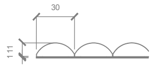
Section View
